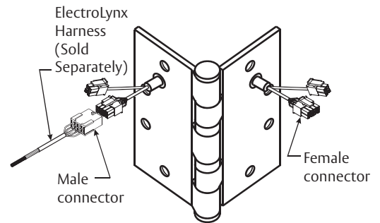
Back of 12 wire hinge shown
