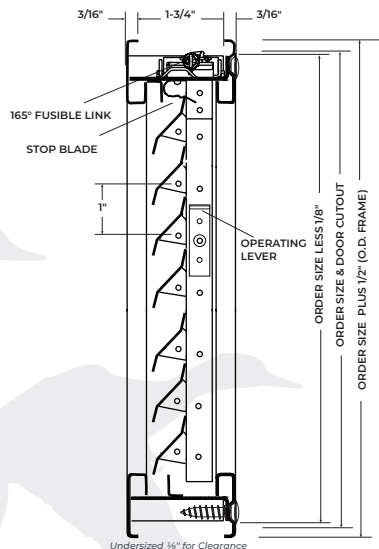
Top View Fusible Link Mechanism
