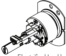
Electrified Lockbody 1-3/8" - 2" Door
