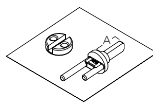
10-3773 (A=0.635") 10-3774 (A=0.798")
